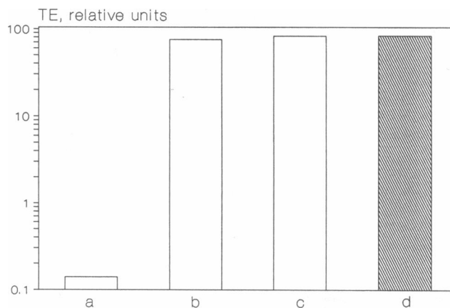
FIGURE 3 Effect of DNAase on transfection efficiency of Cos-1 cells. DNAase (to 5 mg/ml) and MgCl_2 (to 5 mM) were added to cell suspension 3 s before (a), within 3 s (b), and 20 s after (c) the pulse delivery; (d) only MgCl_2 added. Other experimental conditions as described in the legend to Fig. 1.
