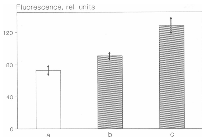
FIGURE 7 Increase in cell membrane permeability for Lucifer Yellow (LY) after electric field treatment in the presence of DNA of different size. 1.5 \times 10^6 Cos-1 cells in 100 \mu l PBS were subjected to 3.5 kV/cm, 100 \mu s pulse in the presence of equimolar concentration of plasmid pCH110 (7.2 kb) or phage \lambda DNA (48 kb) and 5 min after LY was added to 3 mM concentration. After subsequent incubation for 10 min, 300 \mu l of growth medium with serum was added and the cells were allowed to stay for 30 min at 25°C (resealing time). Then the cells were washed carefully and the amount of LY entrapped was measured. See Materials and Methods for details. (a) No DNA in the sample; (b) pCH110, 10 \mu g/ml; (c) phage \lambda DNA, 67 \mu g/ml. Fluorescence intensity of control cells not subjected to electric field is taken as zero.
