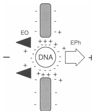
FIGURE 8 The scheme illustrating DNA movement through the hydrophilic pore in the membrane. Electrophoretic force (EPh) moves DNA toward the positive electrode, while the electroosmotic water flux (EO) resulted from the movement of counterions along the negatively charged membrane surface is directed oppositely.
